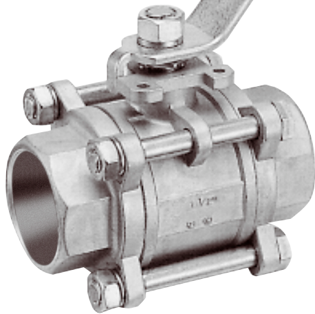
CSC-9603-W carbon steel, socket weld
